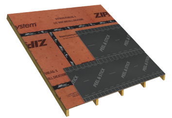
UNDERLAYMENT
