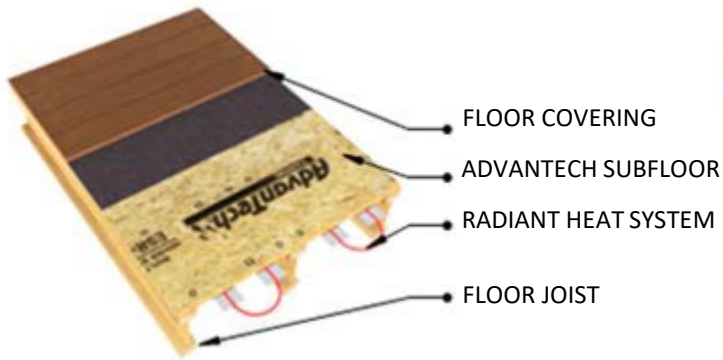
Electric Roll Heating System Below Subfloor
