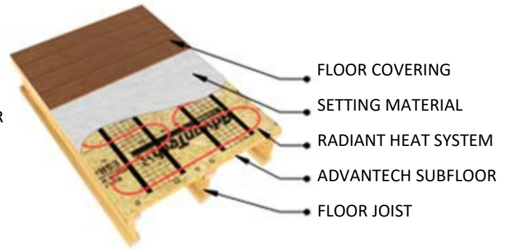
Radiant Heating System Above Subfloor
