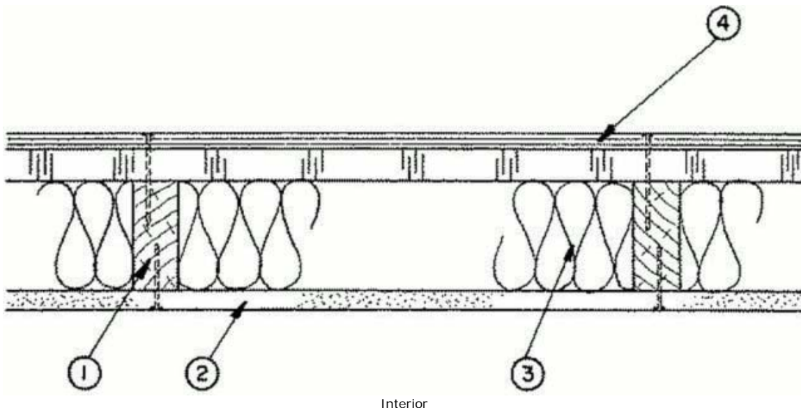
1. Wood Studs — Nom 2 by 4 in., spaced 16 in. OC.
